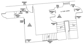
ACCESS STAIR PLAN (1:50) (GROUND TO 1st FLOOR)
